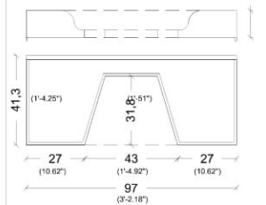
TOP VIEW DRAWER
